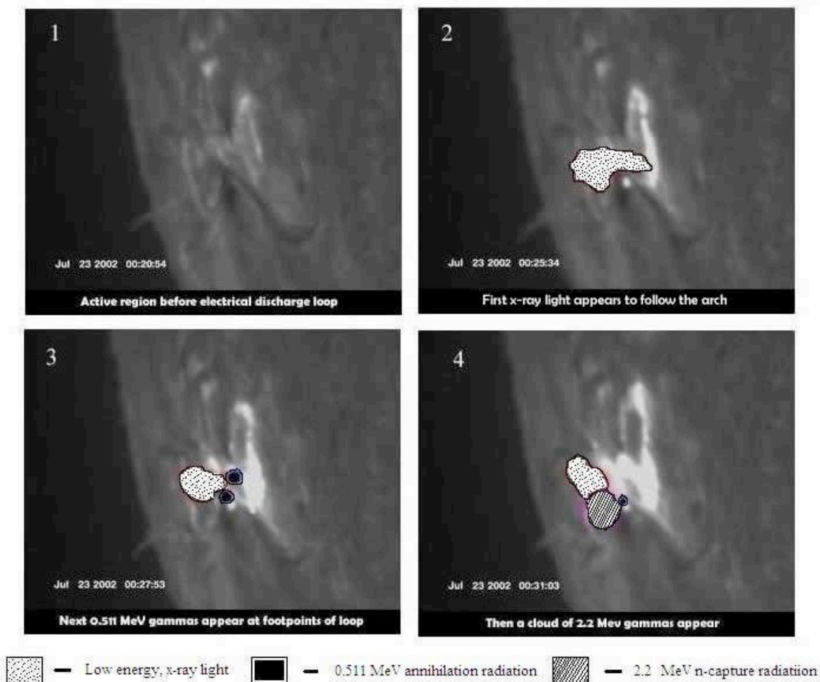
Fig. 2. This shows four sequential animation frames of the solar flare event at Active Region 10039 recorded with a spectrometer on the RHESSI spacecraft on 23 July 2002 [21]. Frame 1 shows the area at 00:20:54. Frame 2 shows the area 4 min and 40 sec later, at 00:25:34, when 12-25 keV x-rays appear along the discharge loop. Frame 3 shows the area almost 7 min after the first frame, at 00:27:53, when 0.511 MeV \gamma 's appear as dark footpoints of the discharge loop. Frame 4 shows the area 10 min and 9 sec after the first frame, when 2.223 MeV \gamma 's reveal a region where hydrogen is undergoing neutron-capture.
